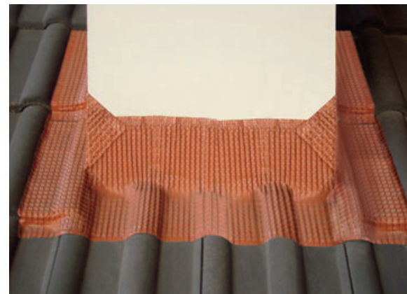
Flue-to-roof transition area
